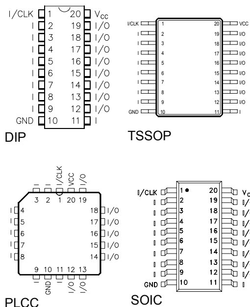
Figure 2 Pin Configuration
