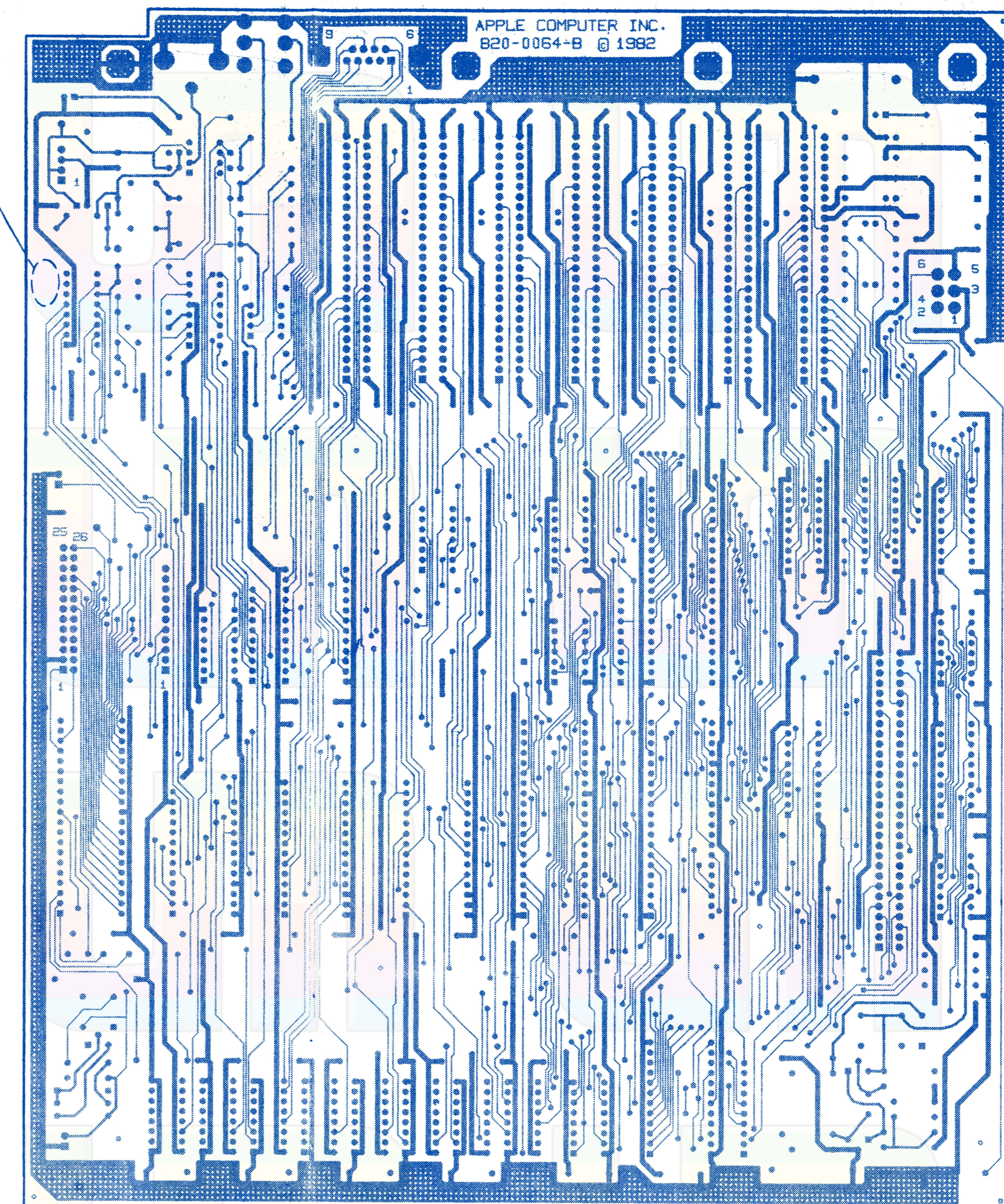
NON-COMPONENT SIDE
