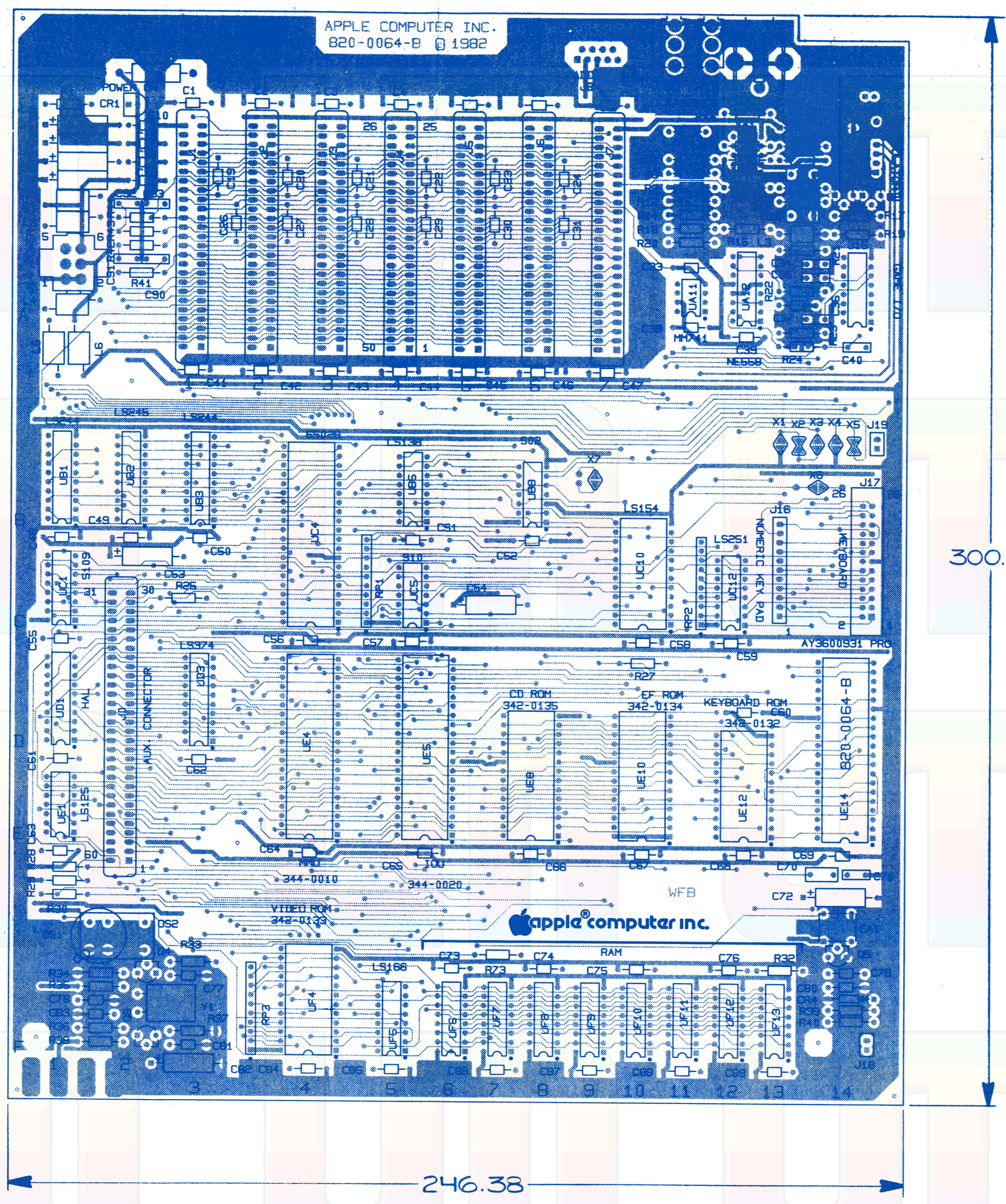
COMPONENT SIDE
